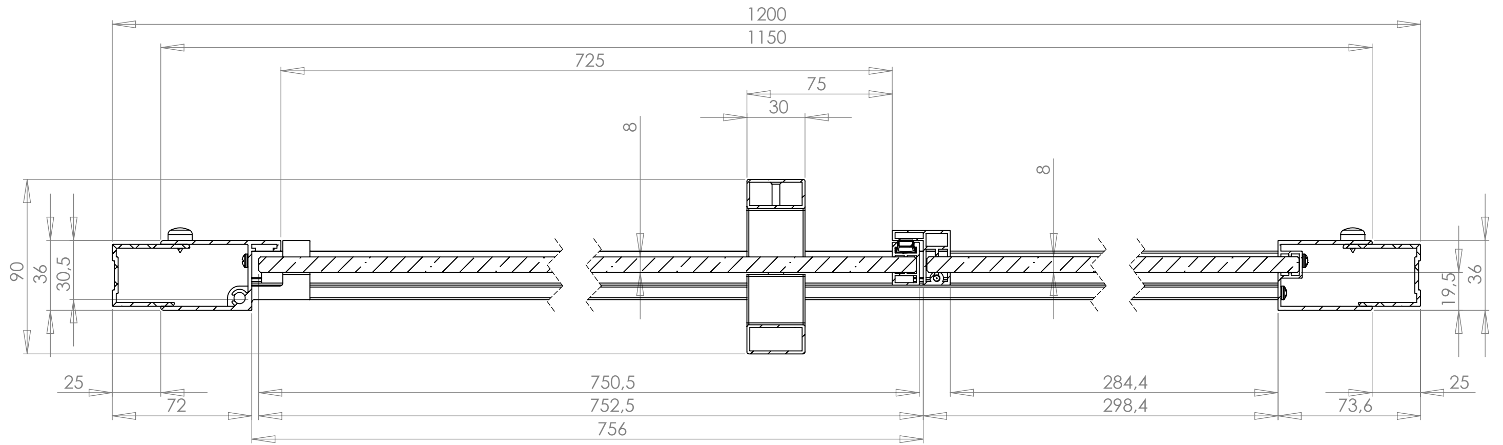
SECTION C-C SCALE 1 : 2
